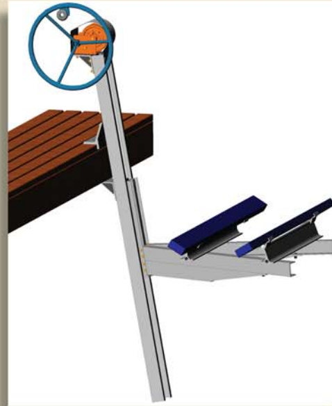
Diagonal installation
